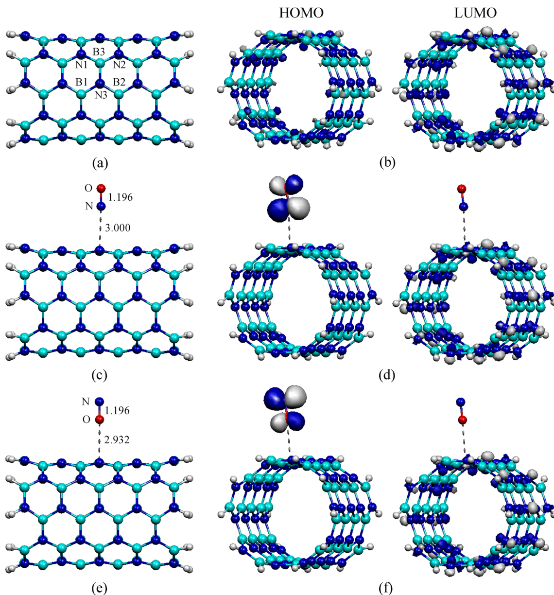
Fig. 1 The B3LYP/LanL2DZ optimized structures of a pristine BNNT, c \underline{\text{NO}} , and e \underline{\text{NO}} adsorbed on pristine BNNT and the plots of HOMO and LUMO density distributions of b pristine BNNT, d \underline{\text{NO}} , and f \underline{\text{NO}} adsorbed on pristine BNNT. Bond lengths and adsorption distances are in Å
