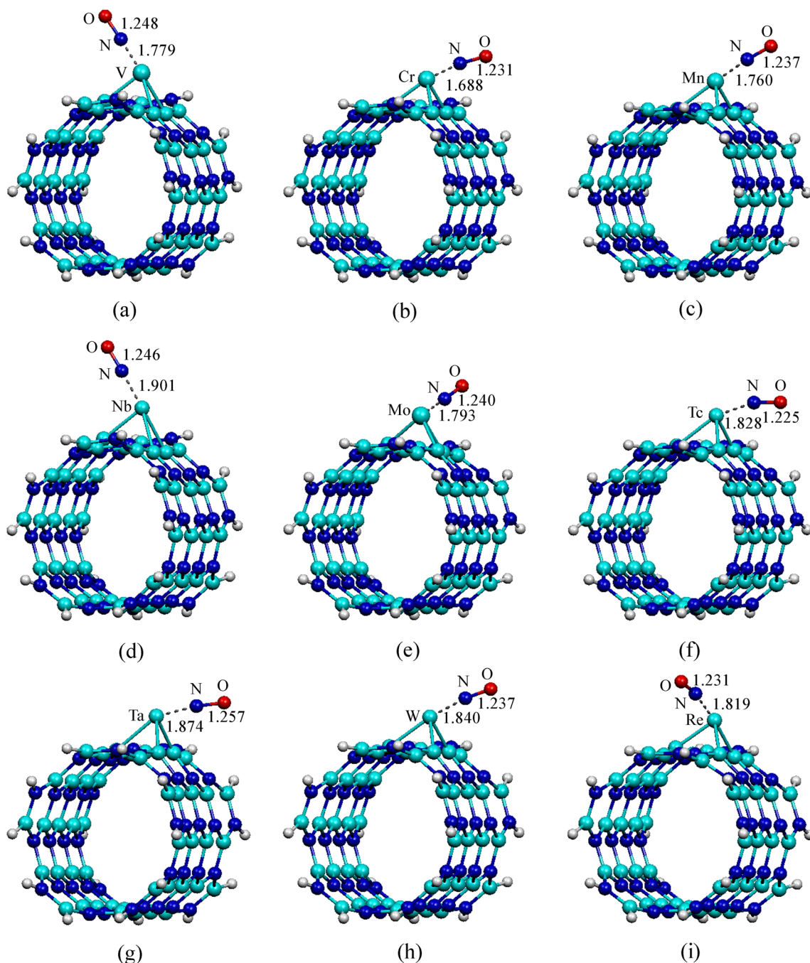
Fig. 5 The B3LYP/LanL2DZ optimized structures of a \underline{\text{NO}}/\text{V}_{\text{N}} -, b \underline{\text{NO}}/\text{Cr}_{\text{N}} -, c \underline{\text{NO}}/\text{Mn}_{\text{N}} -, d \underline{\text{NO}}/\text{Nb}_{\text{N}} -, e \underline{\text{NO}}/\text{Mo}_{\text{N}} -, f \underline{\text{NO}}/\text{Tc}_{\text{N}} -, g \underline{\text{NO}}/\text{Ta}_{\text{N}} -, h \underline{\text{NO}}/\text{W}_{\text{N}} -, and i \underline{\text{NO}}/\text{Re}_{\text{N}} -doped BNNTs
