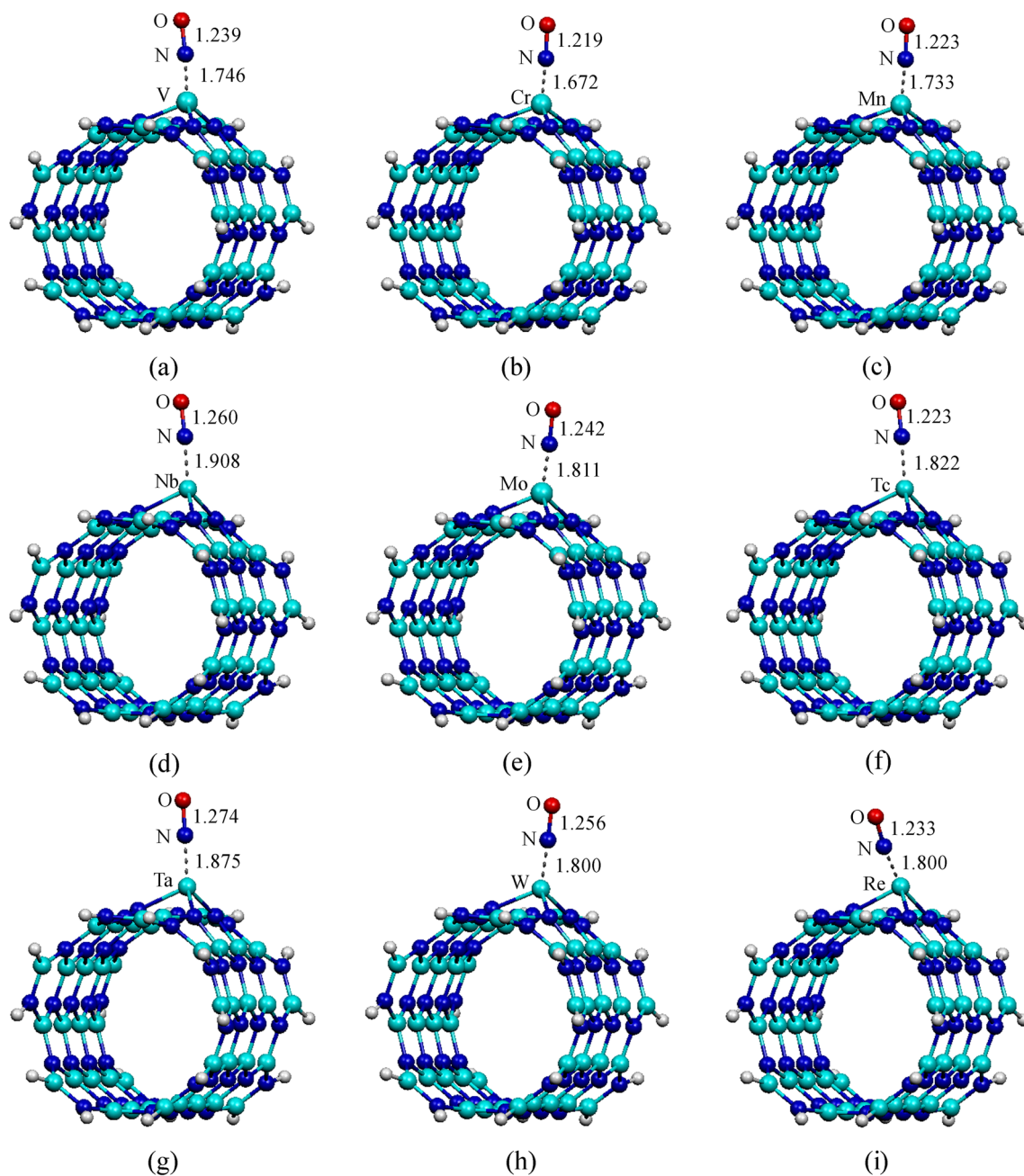
Fig. 4 The B3LYP/LanL2DZ optimized structures of a \underline{\text{NO}}/\text{V}_{\text{B}} , b \underline{\text{NO}}/\text{Cr}_{\text{B}} , c \underline{\text{NO}}/\text{Mn}_{\text{B}} , d \underline{\text{NO}}/\text{Nb}_{\text{B}} , e \underline{\text{NO}}/\text{Mo}_{\text{B}} , f \underline{\text{NO}}/\text{Tc}_{\text{B}} , g \underline{\text{NO}}/\text{Ta}_{\text{B}} , h \underline{\text{NO}}/\text{W}_{\text{B}} , and i \underline{\text{NO}}/\text{Re}_{\text{B}} -doped BNNTs
