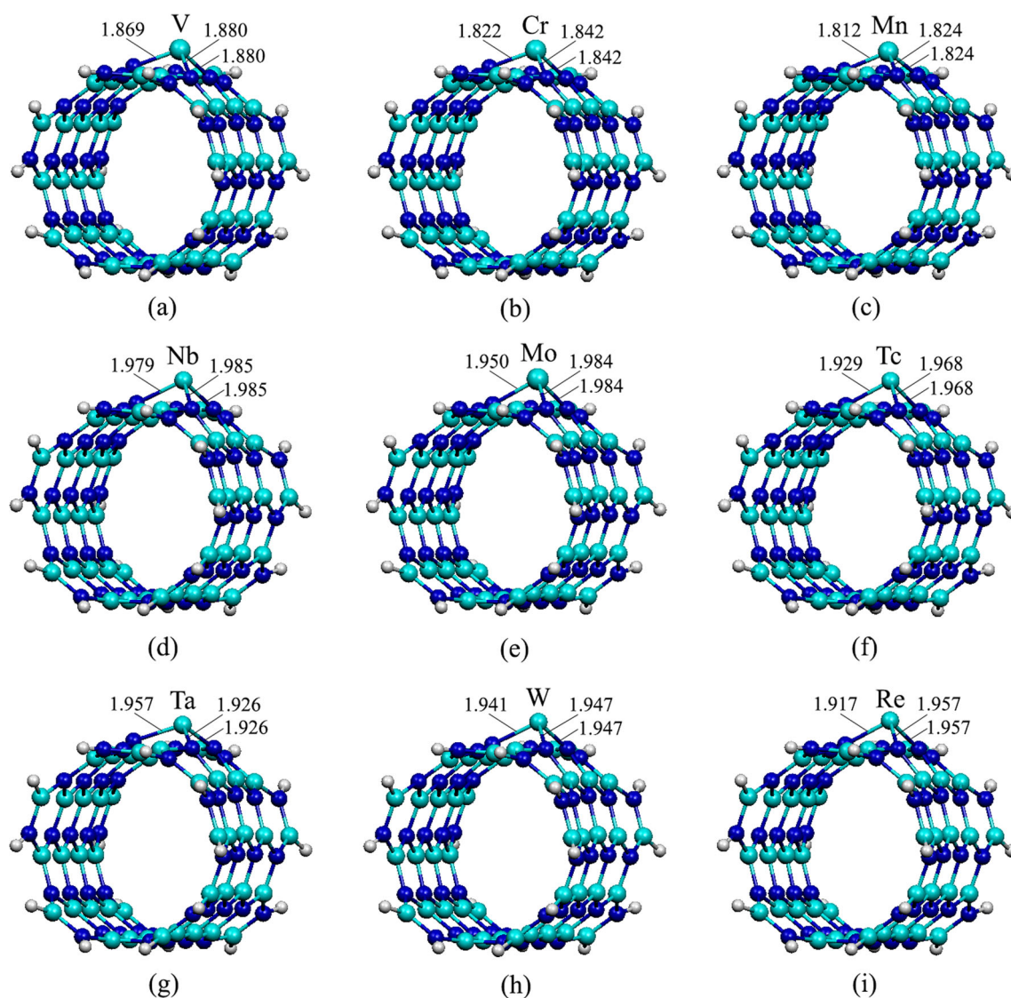
Fig. 2 The B3LYP/LanL2DZ optimized structures of a V B -, b Cr B -, c Mn B -, d Nb B -, e Mo B -, f Tc B -, g Ta B -, h W B -, and i Re B -doped BNNTs
