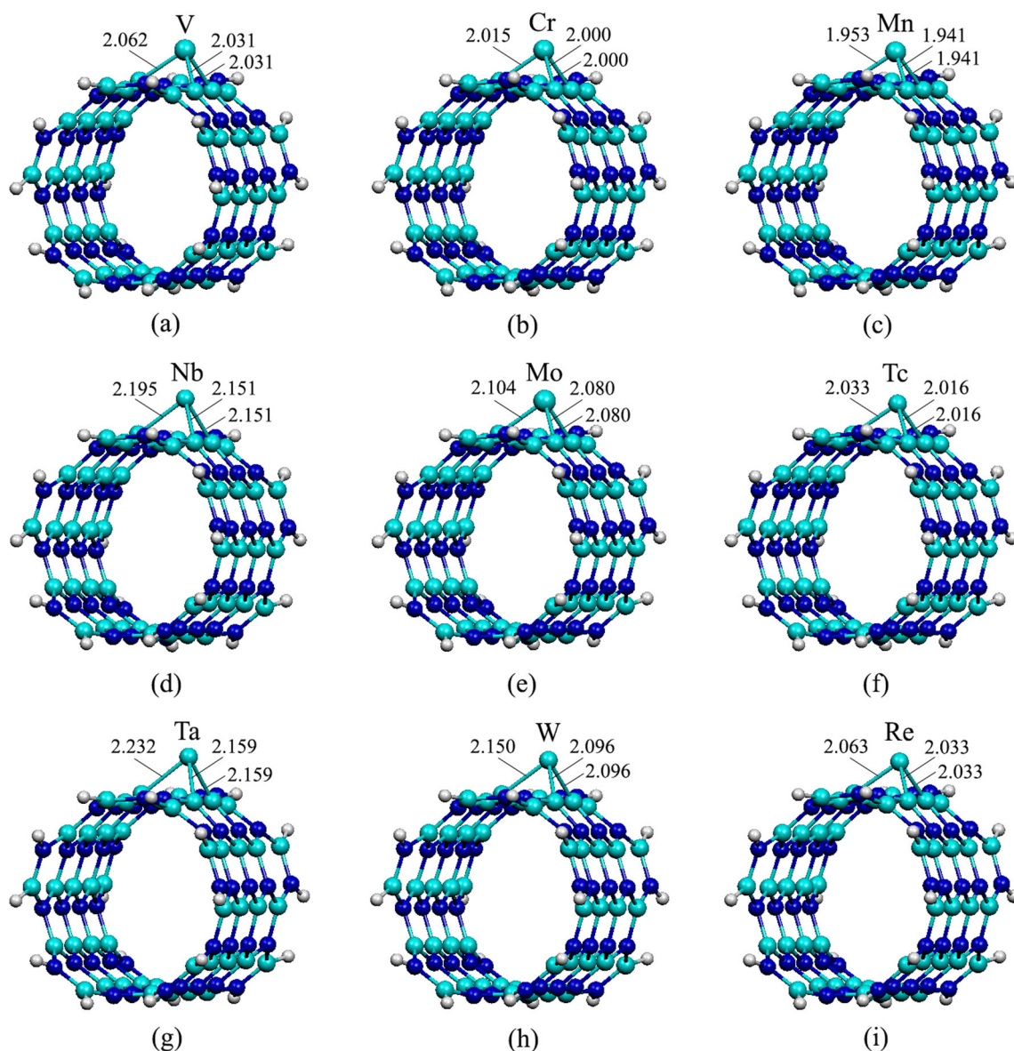
Fig. 3 The B3LYP/LanL2DZ optimized structures of a V N -, b Cr N -, c Mn N -, d Nb N -, e Mo N -, f Tc N -, g Ta N -, h W N -, and i Re N -doped BNNTs
