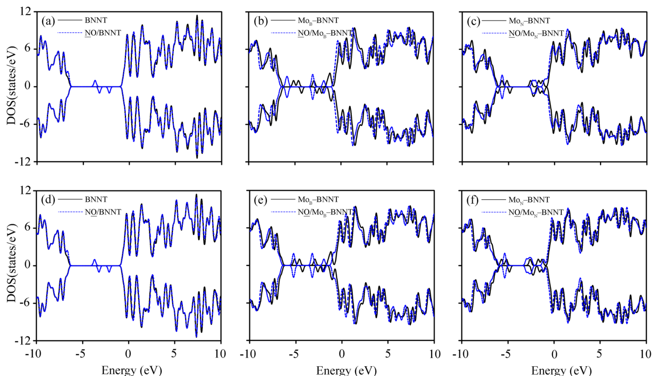
Fig. 8 DOSs of \text{NO} molecule adsorption on a pristine, b \text{Mo}_B , and c \text{Mo}_N -doped BNNTs and DOSs of \text{NO} molecule adsorption on d pristine, e \text{Mo}_B , and f \text{Mo}_N -doped BNNTs
